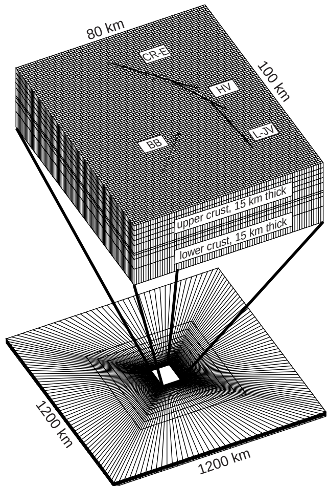
Figure 2. Finite Element Model. The three-dimensional problem domain consists of 109,135 first order elements separated into six layers of poroelastic upper crust elements overlying three layers of viscoelastic lower crust layers.
