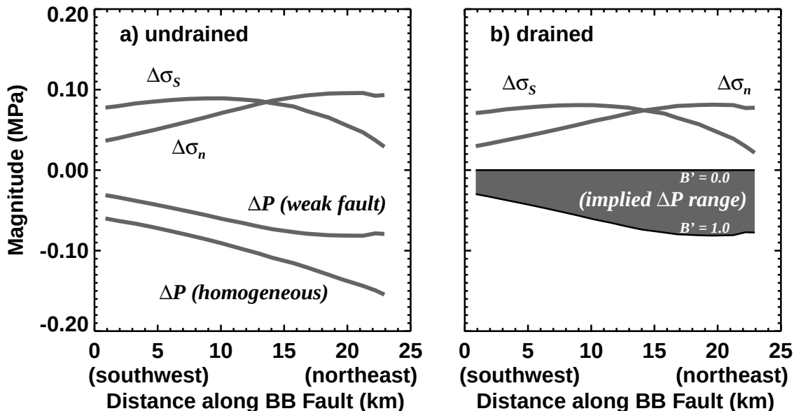
Figure 4. Stress and Pore Pressure Profiles Along the Big Bear Fault. (a) The homogeneous poroelastic and undrained weak fault zone solutions share the same state of stress. However, the magnitude of the homogeneous poroelastic pore pressure decrease is greater than the fault normal stress, therefore the slip potential is significantly smaller compared to the undrained weak fault zone solution. (b) The homogeneous poroelastic pore pressure lies outside of the range implicitly assumed by the drained weak fault zone formulation. For both weak fault zone formulations, the apparent coefficient of friction would have to be less than zero, a nonphysical result.
