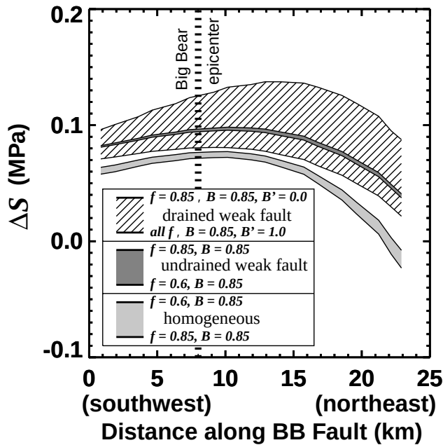
Figure 3. Range of Solutions. Results for each solution method were determined over the frictional range 0.6 \leq f \leq 0.85 . The maximum homogeneous poroelastic solution is most consistent with the location of the epicenter. The weak fault zone solutions do not overlap the homogeneous poroelastic solution. The wide range of possible drained weak fault zone solutions is due to the ambiguity of the parameter B' .
