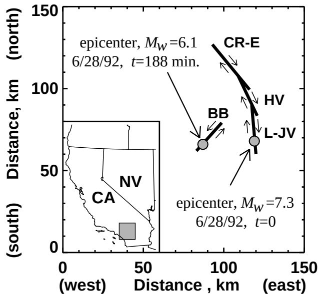
Figure 1. Site Location, 1992 Landers, California Earthquake. The fault trace of the rupture was simplified to include three fault segments designated Camp Rock-Emerson (CR-E), Homestead Valley (HV), and Landers-Johnson Valley (L-JV). The dislocation was primarily right-lateral strike-slip, with up to six meters of offset observed along the 85-kilometer surface trace of the rupture. Left-lateral rupture along the Big Bear (BB) fault occurred 188 minutes later. Although several slip distribution models have been proposed for the Big Bear event, we assume a single 23-kilometer fault striking northeast with an epicenter located seven kilometers from the southwest end.
