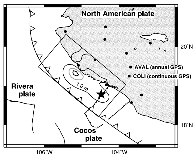
Figure 1. Upper—Tectonic setting and coseismic slip distribution from Hutton et al. [2001]. Rectangle shows surface projection of fault used for elastic half-space and viscoelastic modeling. Contours show coseismic down-dip slip, ranging from 1 meter to 5 meters (bold line). Star shows epicenter of Oct. 9, 1995 Colima-Jalisco earthquake. Circles show locations of GPS sites used to constrain coseismic slip distribution.
